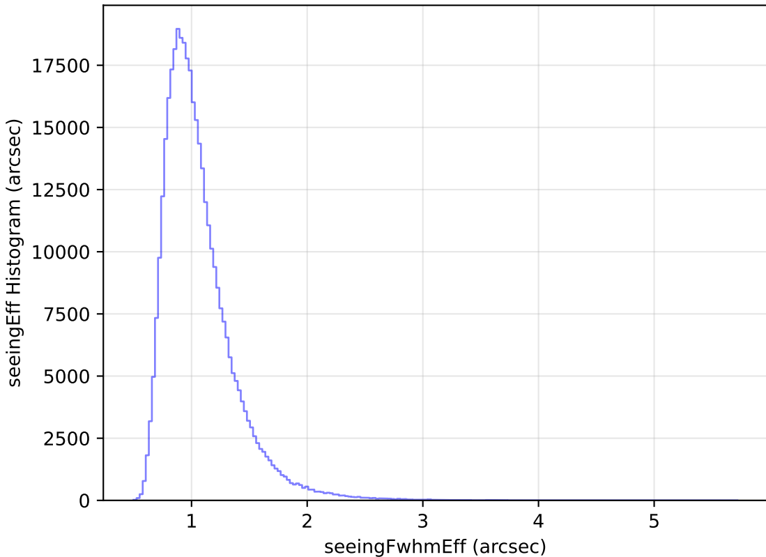
too_elab_r8_d3_griz_v3.4_10yrs WFD y band: seeingEff Histogram
