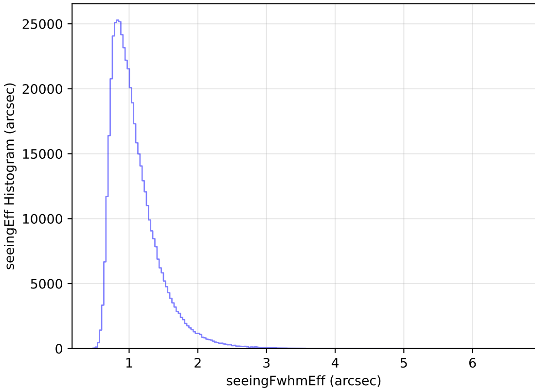
too_elab_r8_d3_griz_v3.4_10yrs WFD i band: seeingEff Histogram
