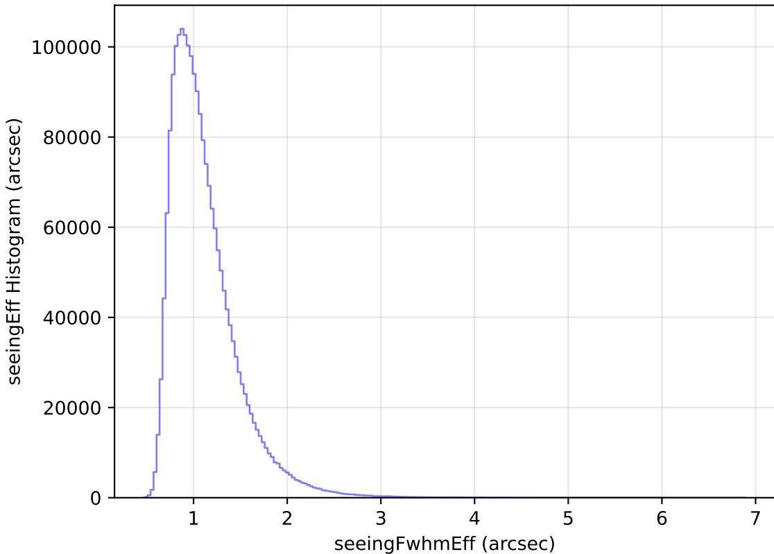
too_elab_r8_d3_griz_v3.4_10yrs WFD all bands: seeingEff Histogram
