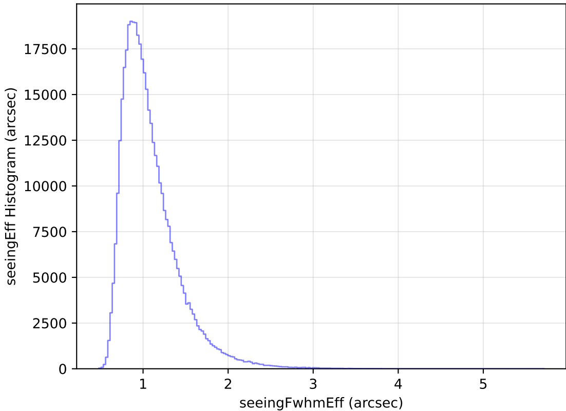
too_elab_r8_d3_griz_v3.4_10yrs All sky z band: seeingEff Histogram
