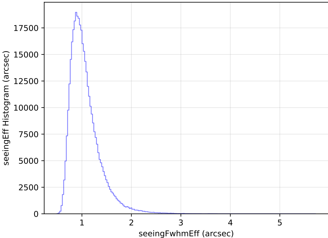
too_elab_r8_d3_griz_v3.4_10yrs All sky y band: seeingEff Histogram
