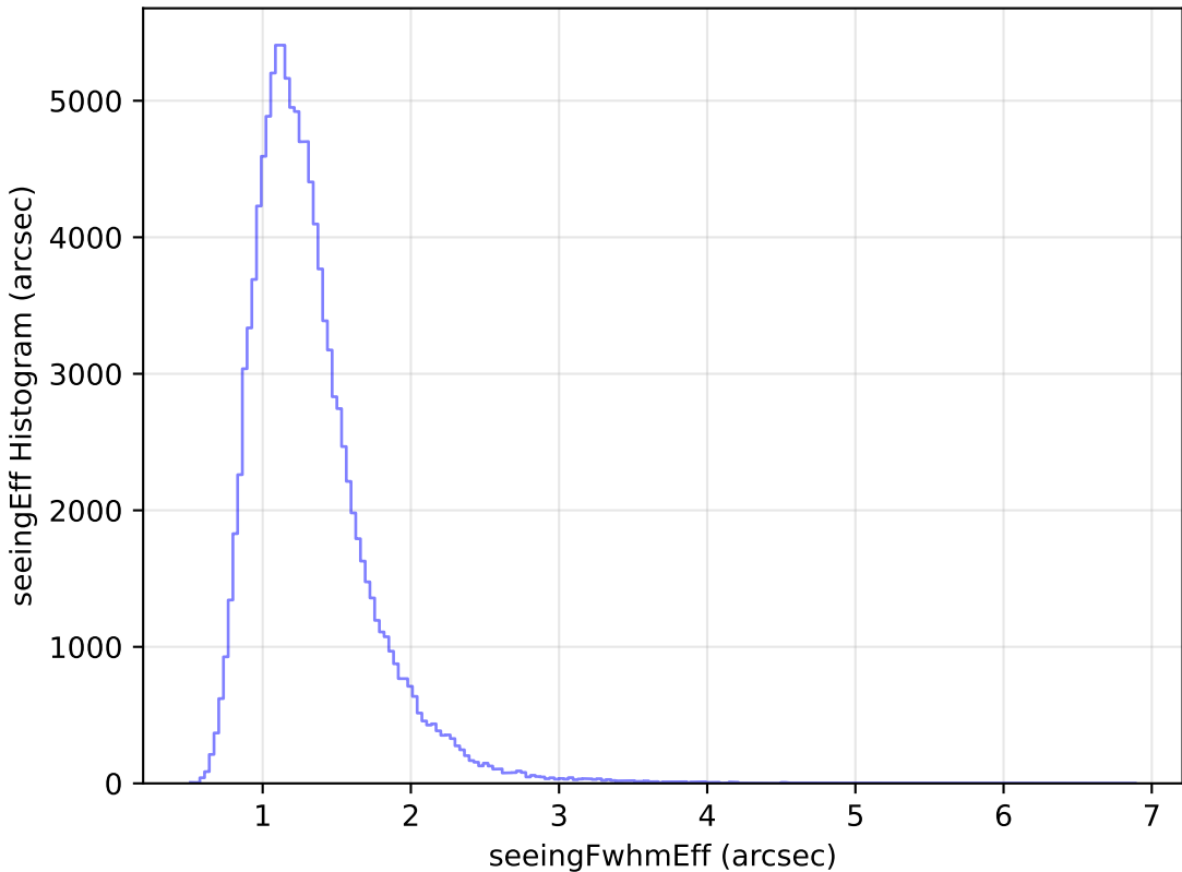
too_elab_r8_d3_griz_v3.4_10yrs All sky u band: seeingEff Histogram
