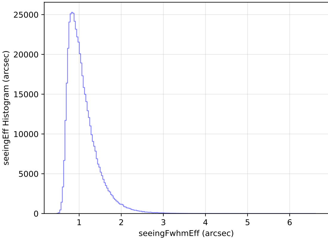
too_elab_r8_d3_griz_v3.4_10yrs All sky i band: seeingEff Histogram
