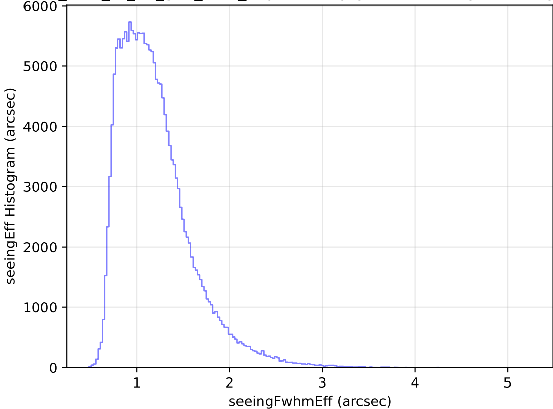
too_elab_r8_d3_griz_v3.4_10yrs All sky g band: seeingEff Histogram
