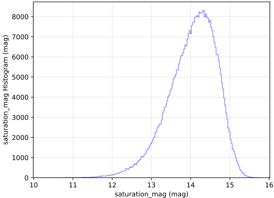
too_elab_r8_d3_griz_v3.4_10yrs WFD z band: saturation_mag Histogram
