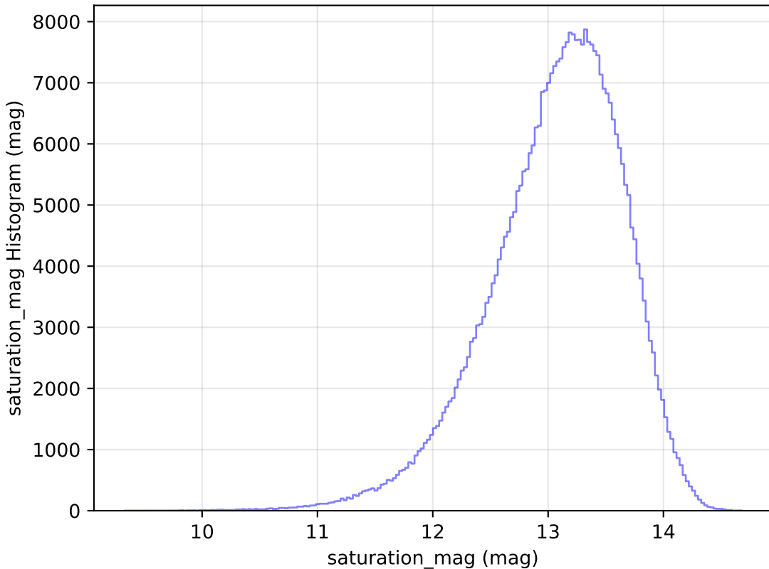
too_elab_r8_d3_griz_v3.4_10yrs WFD y band: saturation_mag Histogram
