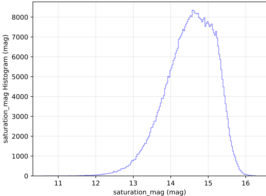
too_elab_r8_d3_griz_v3.4_10yrs WFD r band: saturation_mag Histogram
