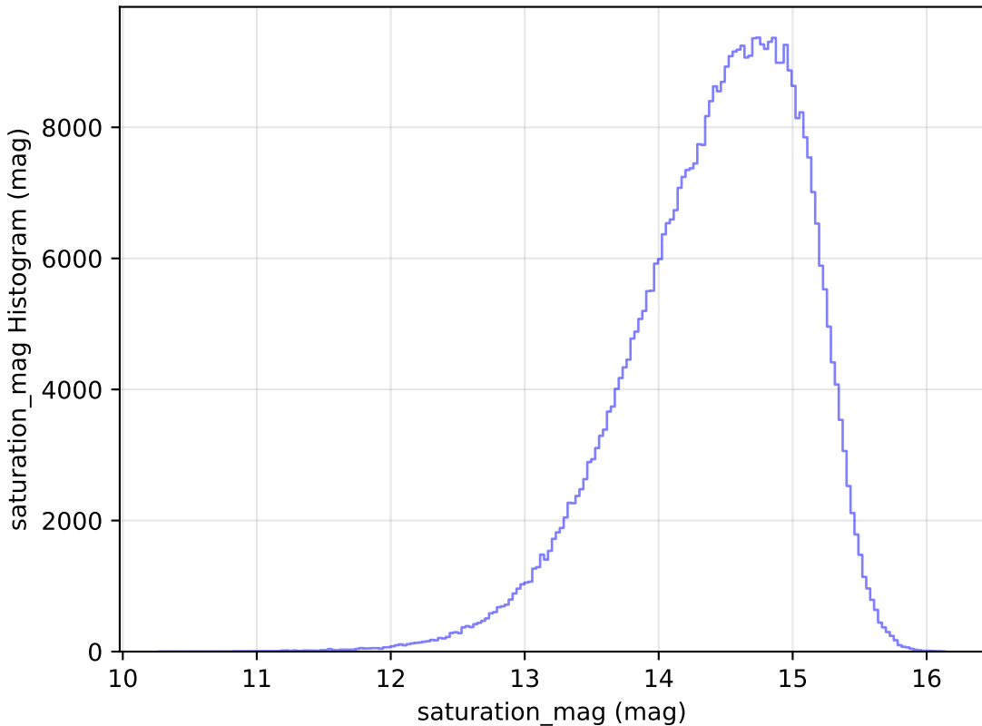
too_elab_r8_d3_griz_v3.4_10yrs WFD i band: saturation_mag Histogram
