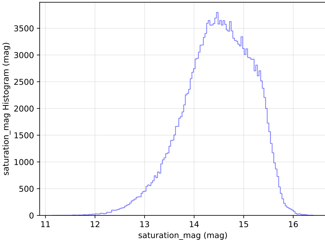
too_elab_r8_d3_griz_v3.4_10yrs WFD g band: saturation_mag Histogram
