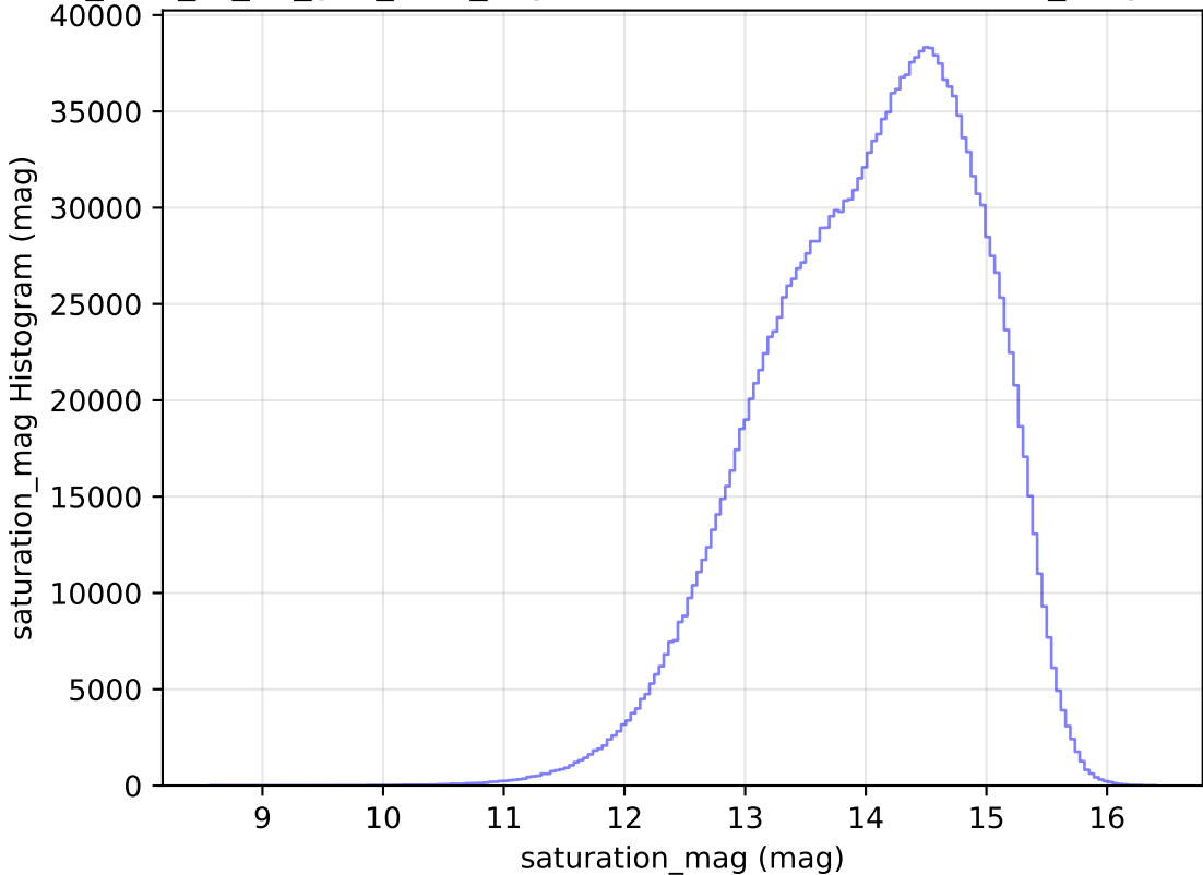
too_elab_r8_d3_griz_v3.4_10yrs WFD all bands: saturation_mag Histogram
