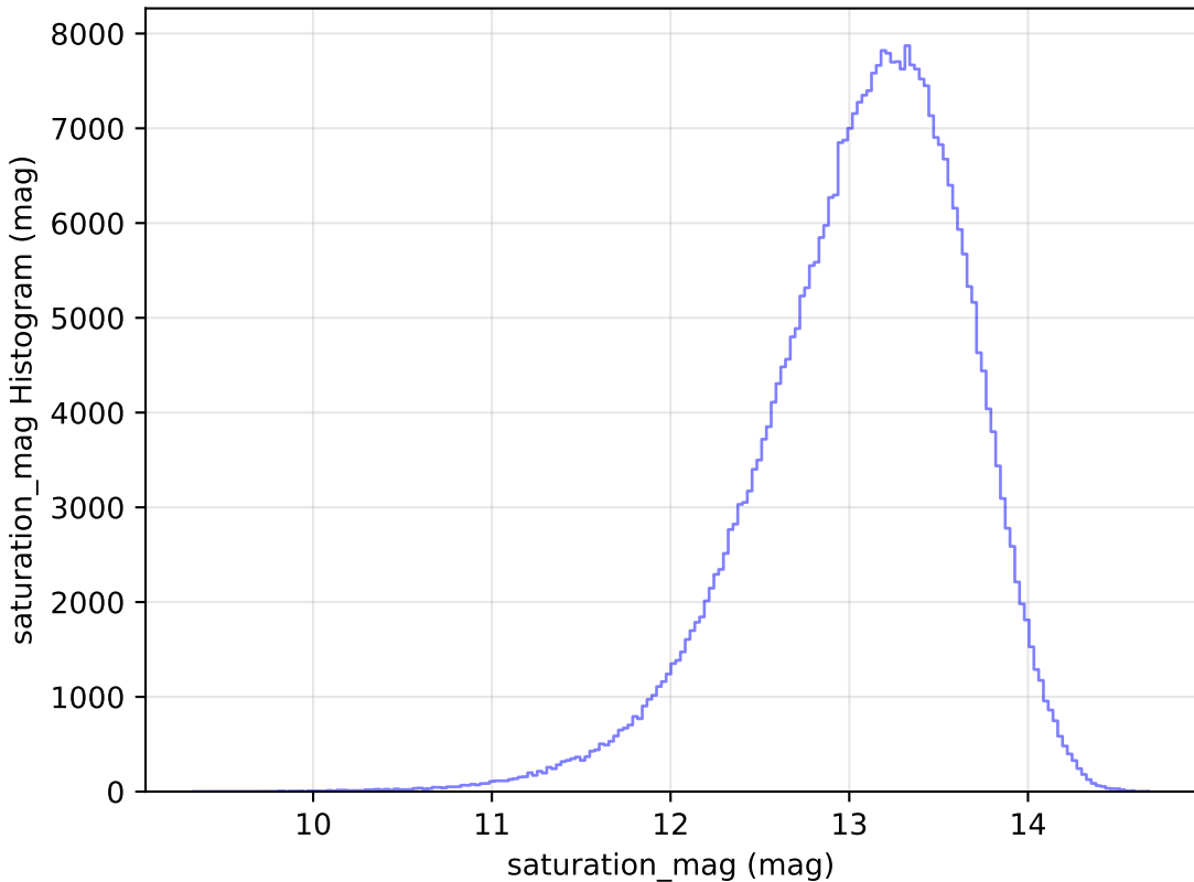
too_elab_r8_d3_griz_v3.4_10yrs All sky y band: saturation_mag Histogram
