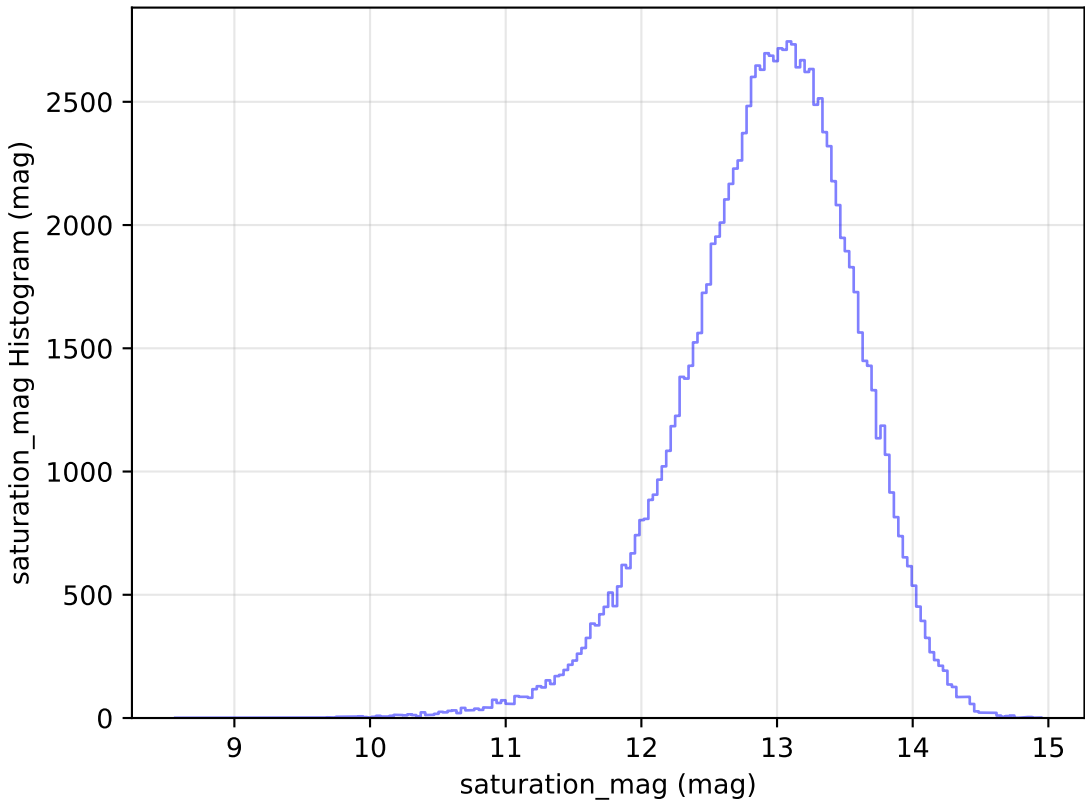
too_elab_r8_d3_griz_v3.4_10yrs All sky u band: saturation_mag Histogram
