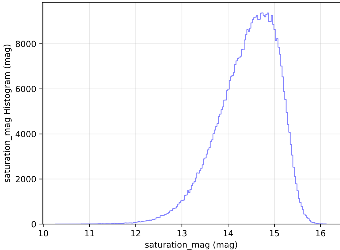
too_elab_r8_d3_griz_v3.4_10yrs All sky i band: saturation_mag Histogram
