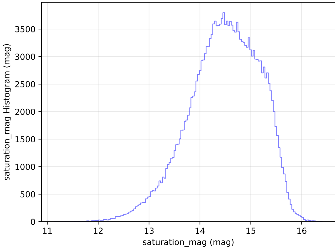
too_elab_r8_d3_griz_v3.4_10yrs All sky g band: saturation_mag Histogram
