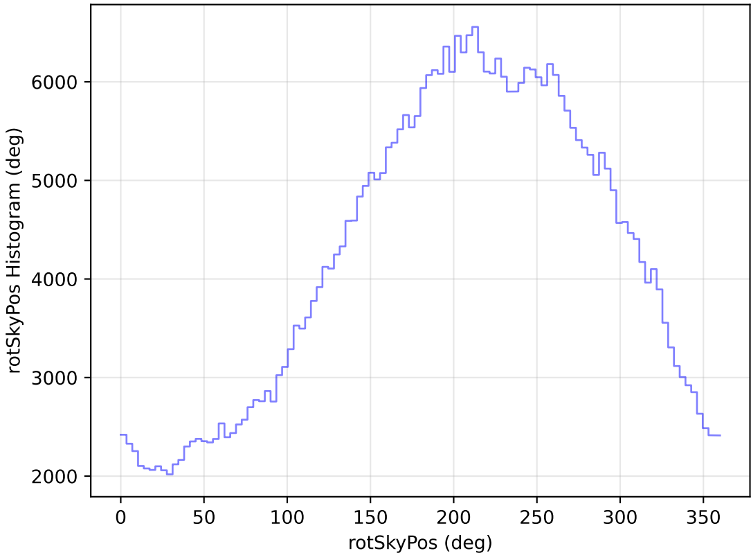
too_elab_r8_d3_griz_v3.4_10yrs WFD z band: rotSkyPos Histogram
