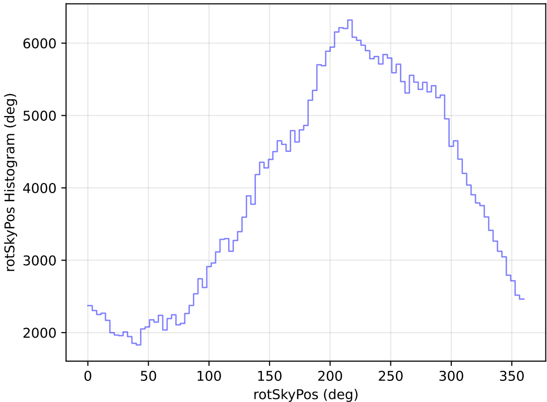
too_elab_r8_d3_griz_v3.4_10yrs WFD y band: rotSkyPos Histogram
