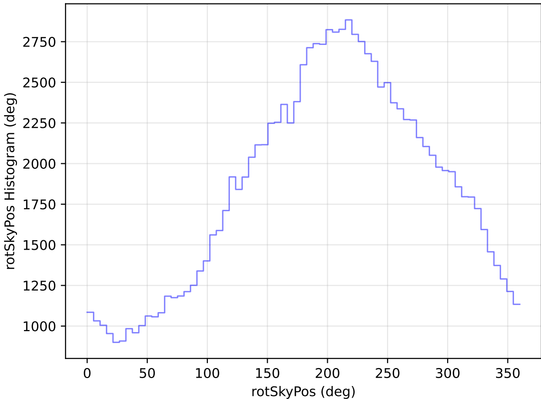
too_elab_r8_d3_griz_v3.4_10yrs WFD u band: rotSkyPos Histogram
