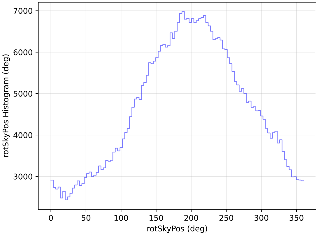
too_elab_r8_d3_griz_v3.4_10yrs WFD r band: rotSkyPos Histogram
