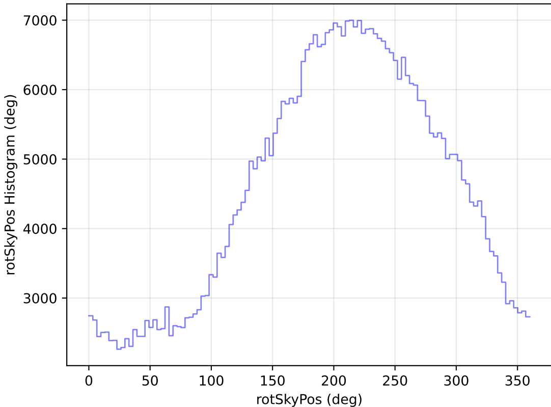
too_elab_r8_d3_griz_v3.4_10yrs WFD i band: rotSkyPos Histogram
