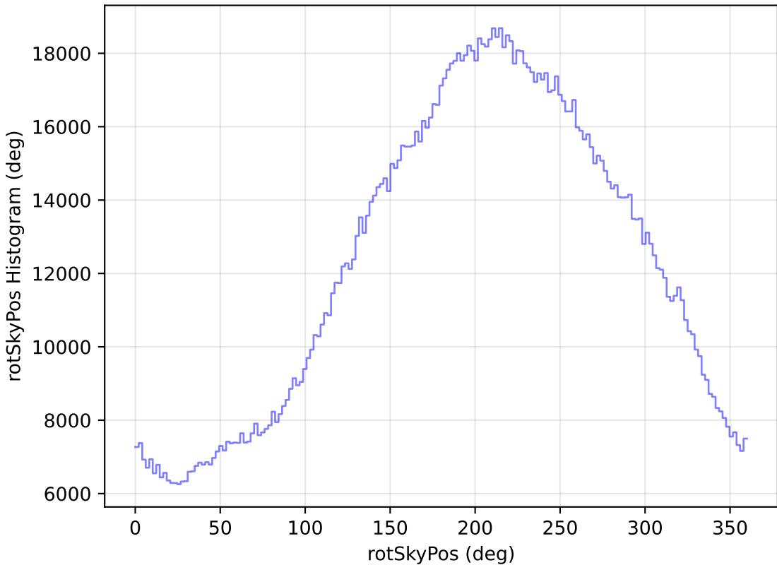
too_elab_r8_d3_griz_v3.4_10yrs WFD all bands: rotSkyPos Histogram
