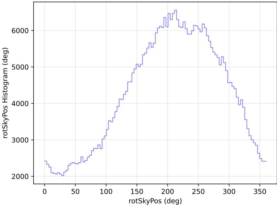
too_elab_r8_d3_griz_v3.4_10yrs All sky z band: rotSkyPos Histogram
