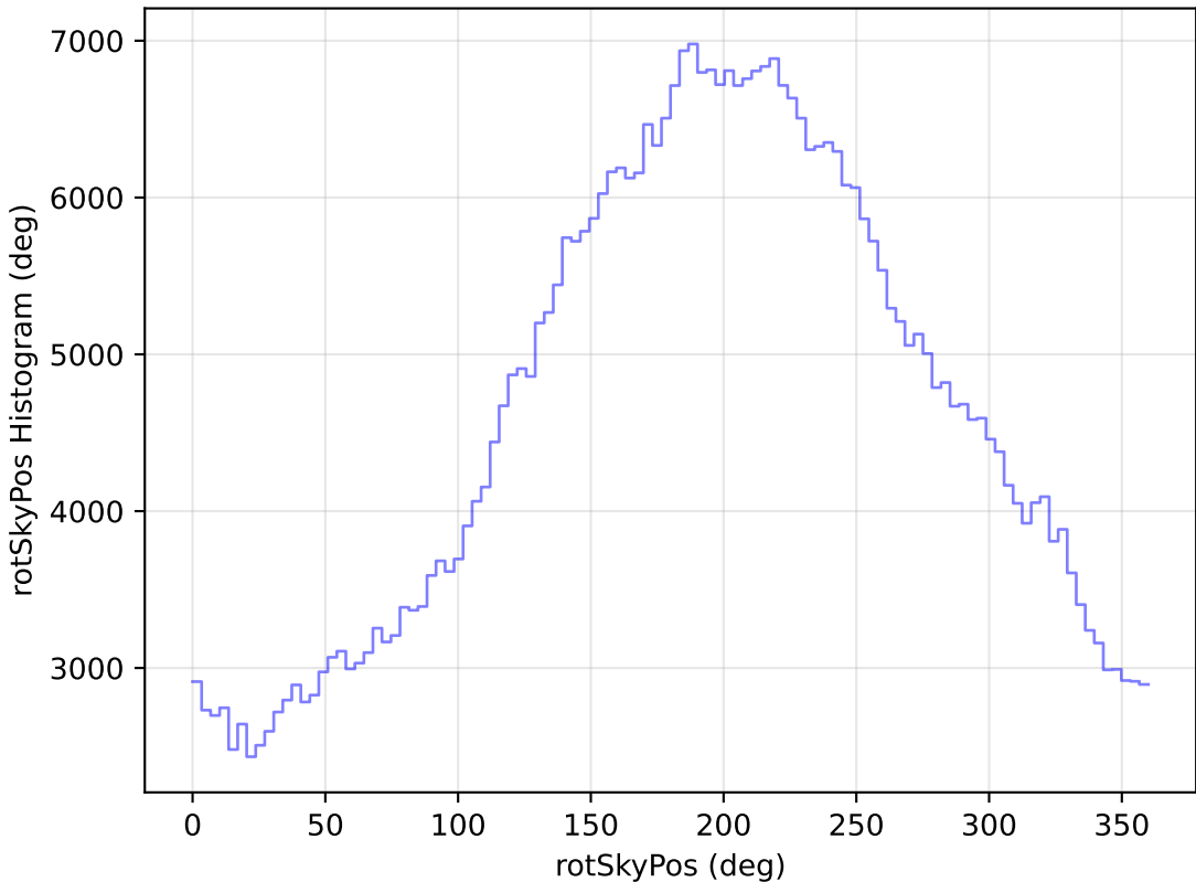
too_elab_r8_d3_griz_v3.4_10yrs All sky r band: rotSkyPos Histogram
