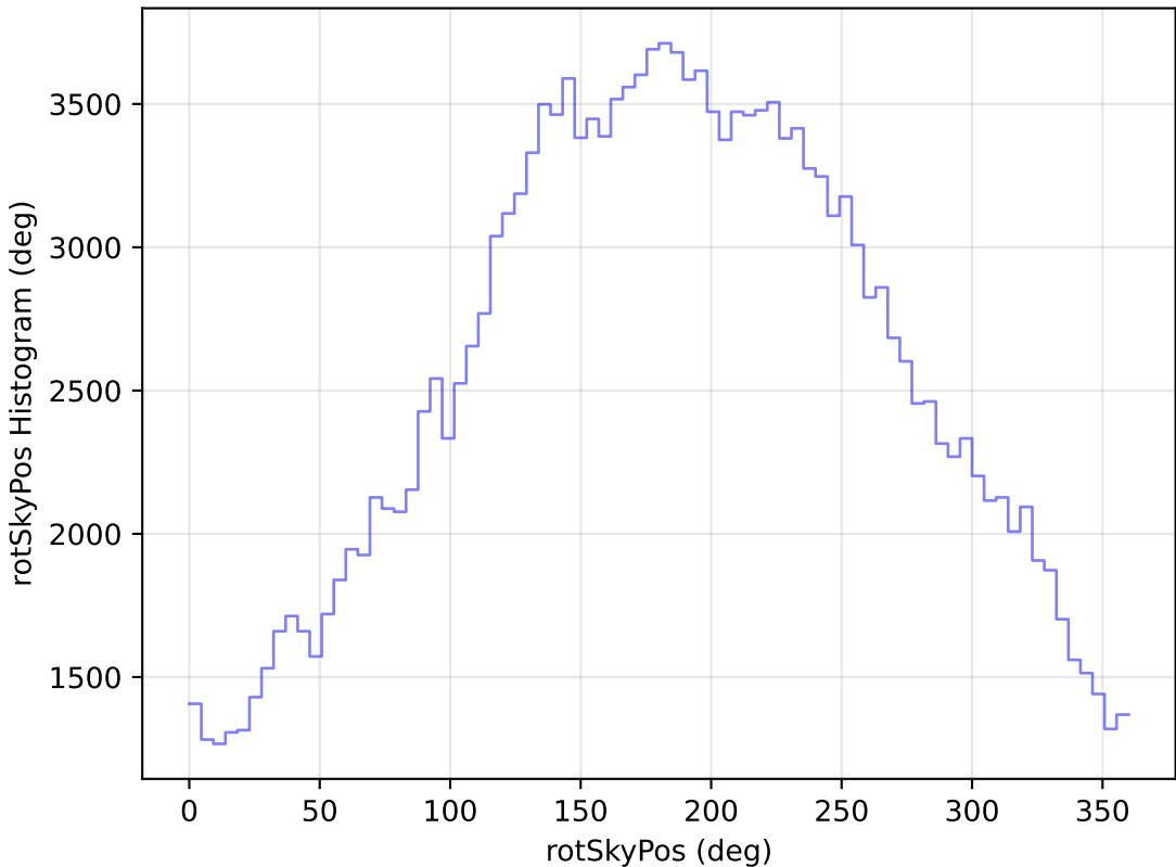
too_elab_r8_d3_griz_v3.4_10yrs All sky g band: rotSkyPos Histogram
