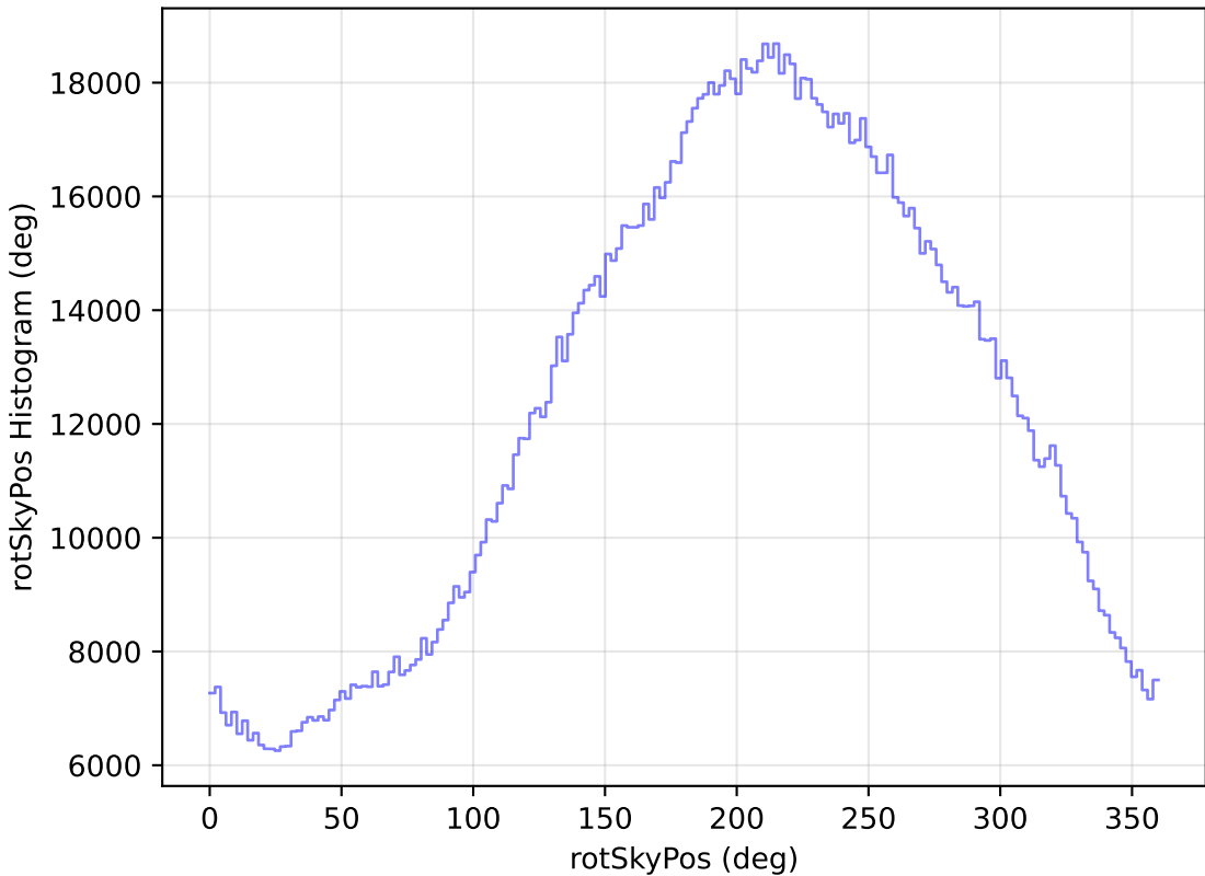
too_elab_r8_d3_griz_v3.4_10yrs All sky all bands: rotSkyPos Histogram
