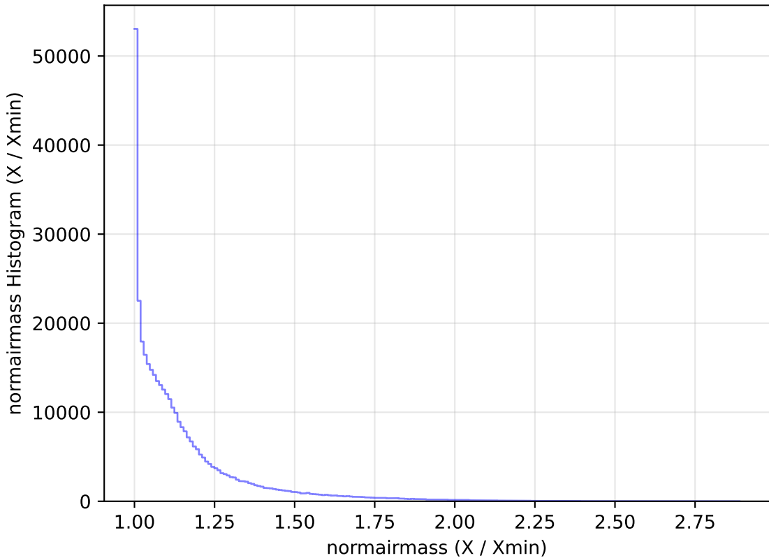
too_elab_r8_d3_griz_v3.4_10yrs WFD y band: normairmass Histogram
