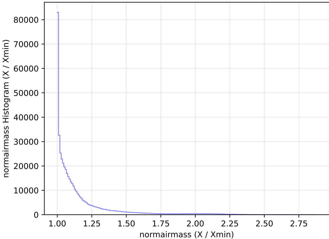
too_elab_r8_d3_griz_v3.4_10yrs WFD r band: normairmass Histogram
