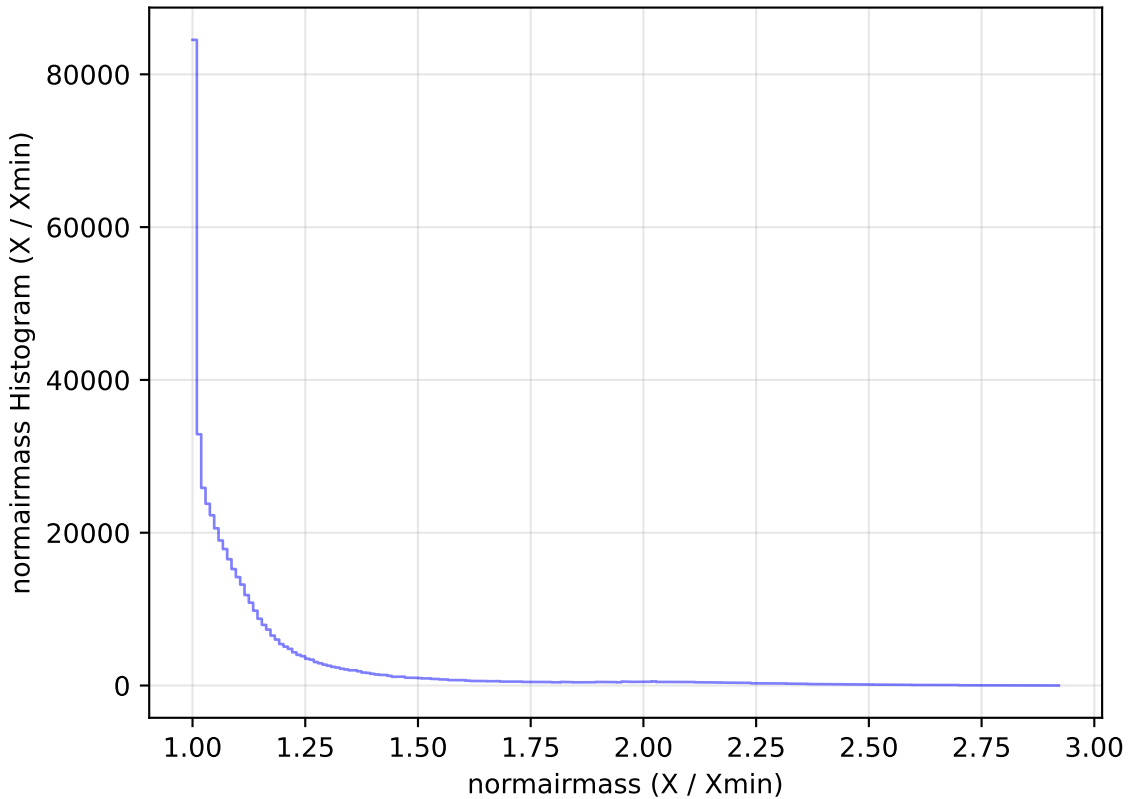
too_elab_r8_d3_griz_v3.4_10yrs WFD i band: normairmass Histogram
