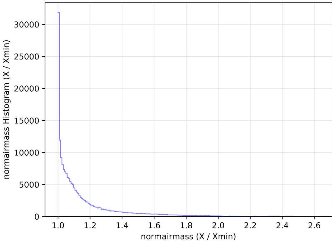
too_elab_r8_d3_griz_v3.4_10yrs WFD g band: normairmass Histogram
