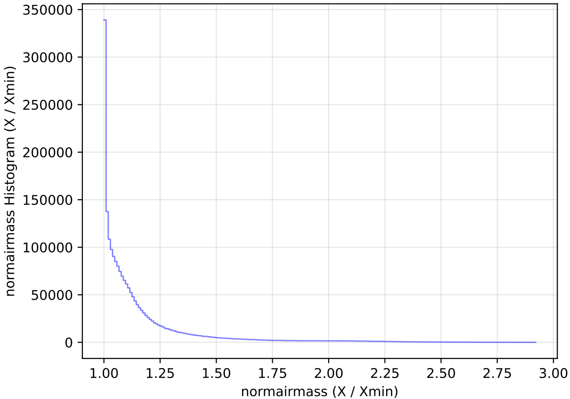
too_elab_r8_d3_griz_v3.4_10yrs WFD all bands: normairmass Histogram
