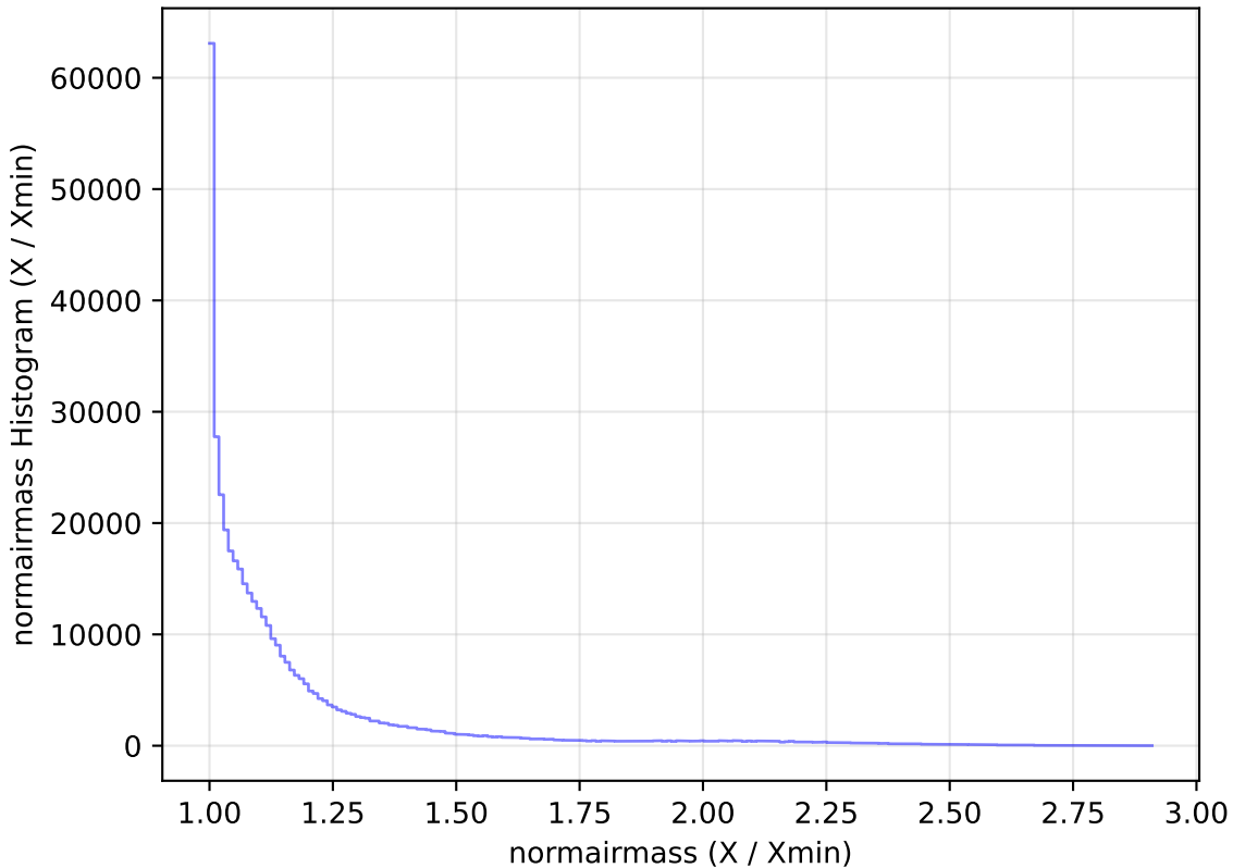
too_elab_r8_d3_griz_v3.4_10yrs All sky z band: normairmass Histogram
