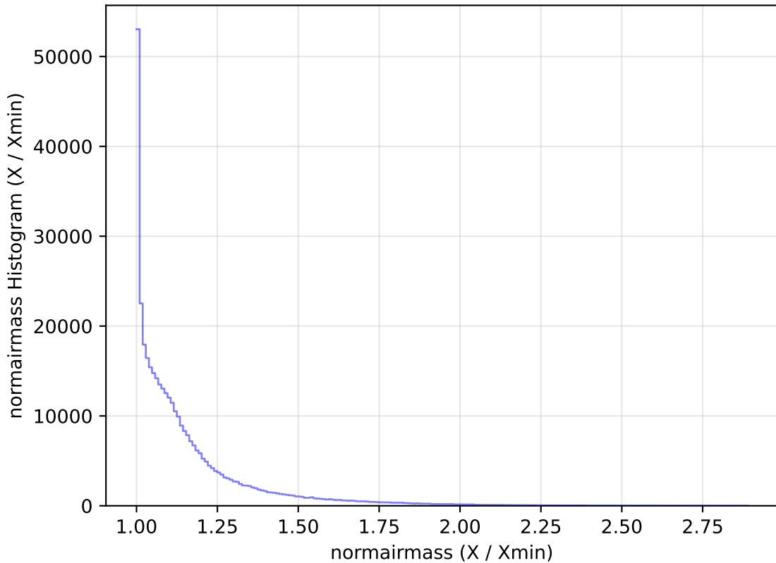
too_elab_r8_d3_griz_v3.4_10yrs All sky y band: normairmass Histogram
