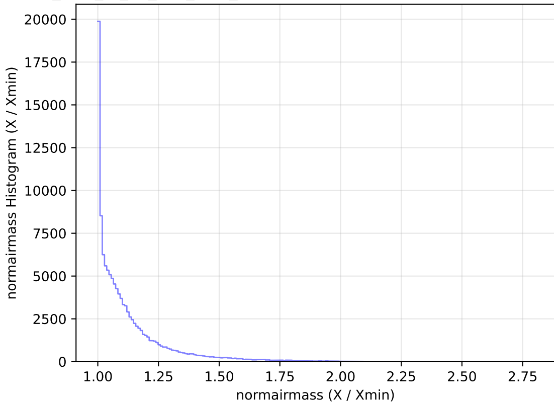
too_elab_r8_d3_griz_v3.4_10yrs All sky u band: normairmass Histogram
