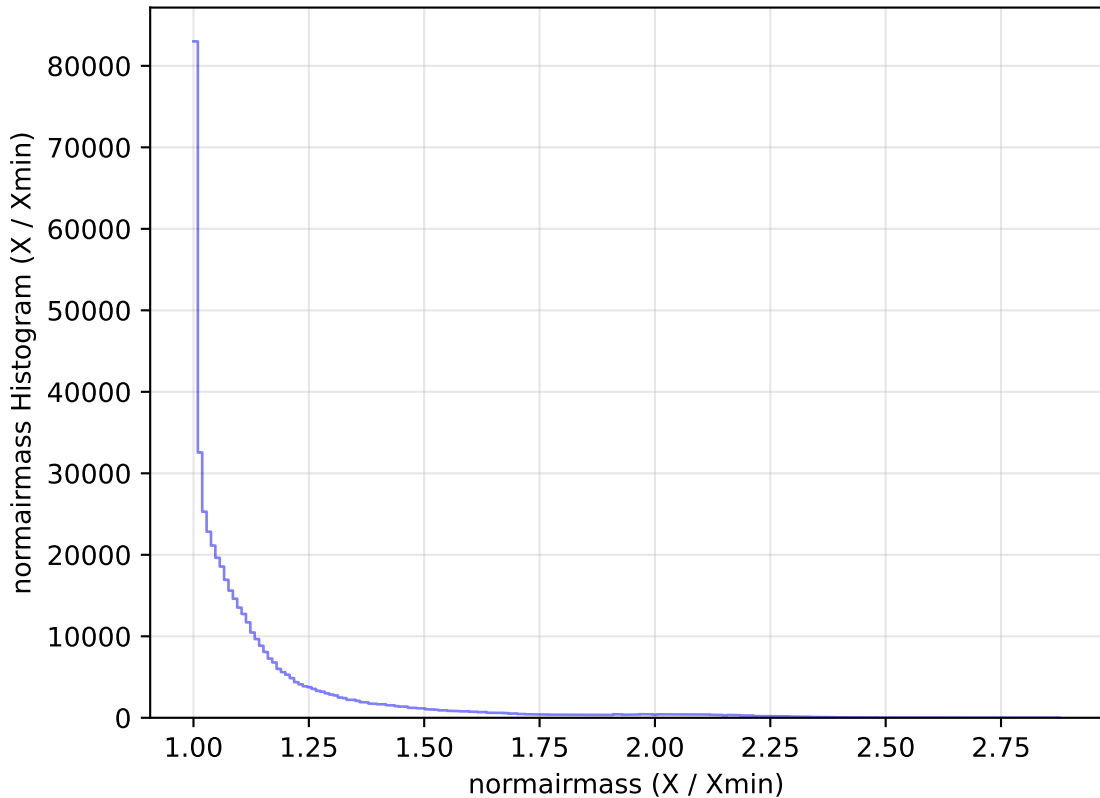
too_elab_r8_d3_griz_v3.4_10yrs All sky r band: normairmass Histogram
