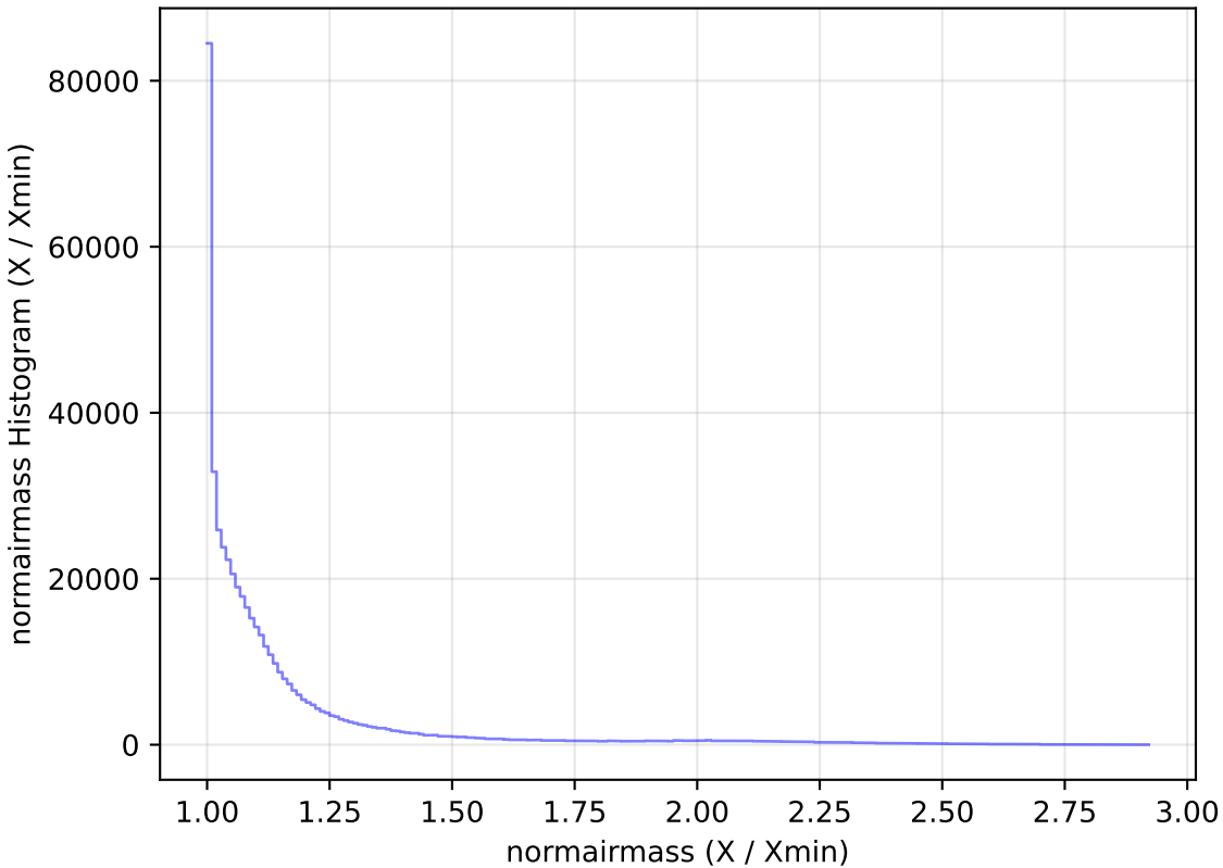
too_elab_r8_d3_griz_v3.4_10yrs All sky i band: normairmass Histogram
