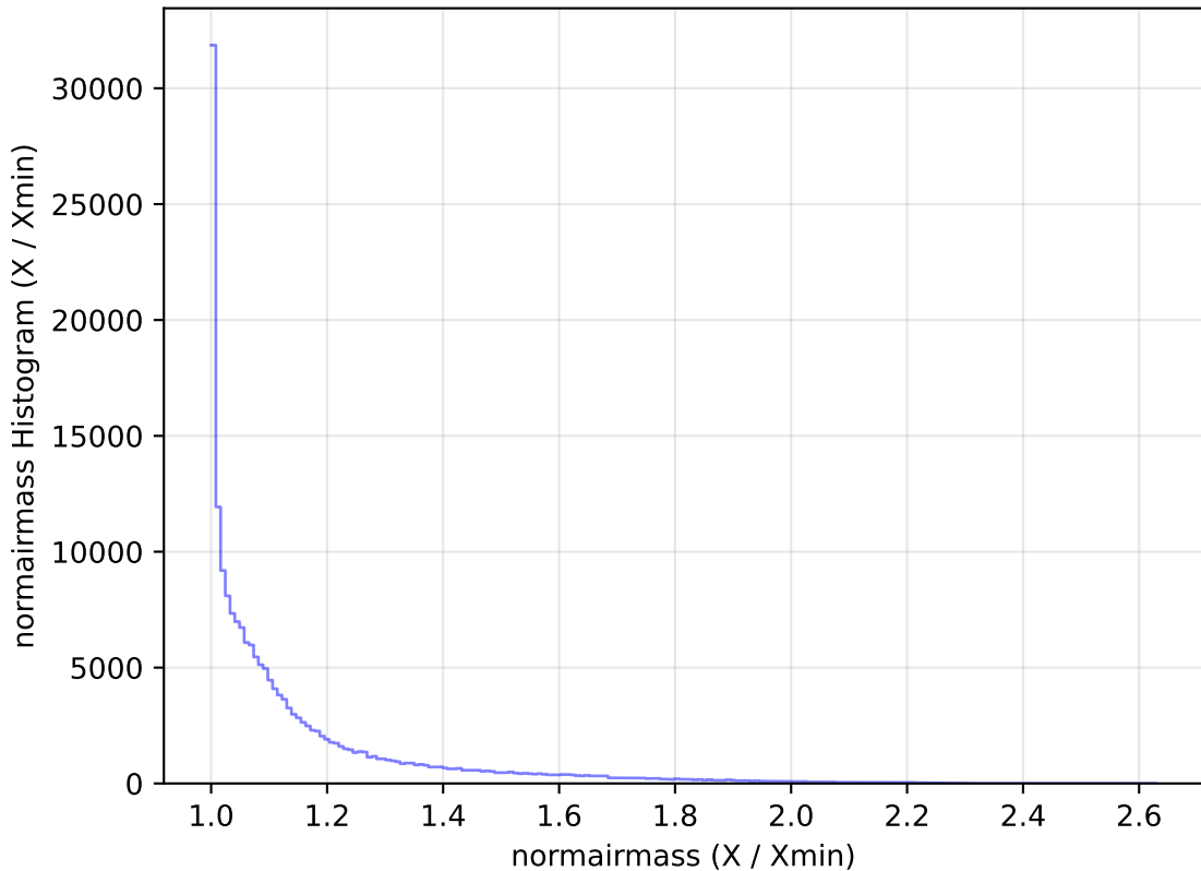
too_elab_r8_d3_griz_v3.4_10yrs All sky g band: normairmass Histogram
