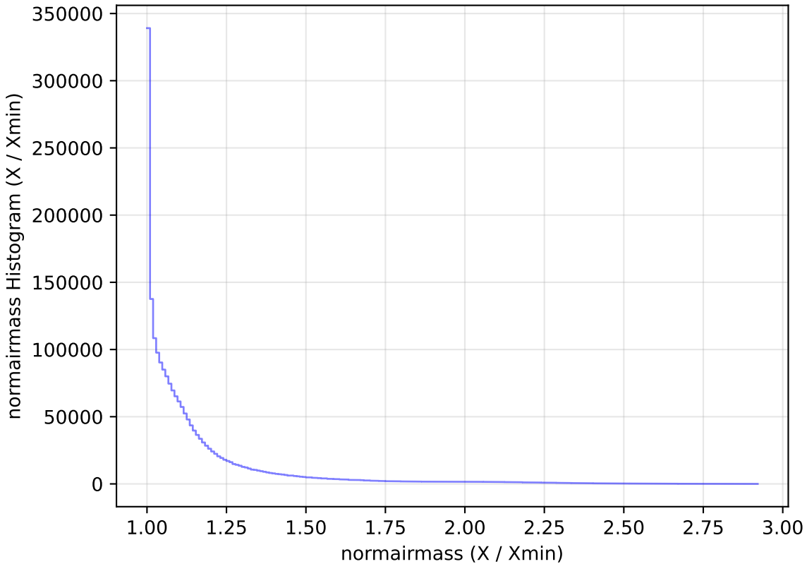
too_elab_r8_d3_griz_v3.4_10yrs All sky all bands: normairmass Histogram
