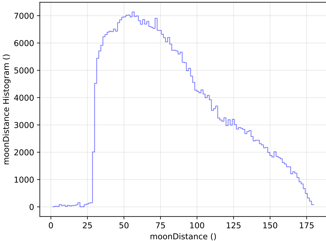
too_elab_r8_d3_griz_v3.4_10yrs WFD z band: moonDistance Histogram
