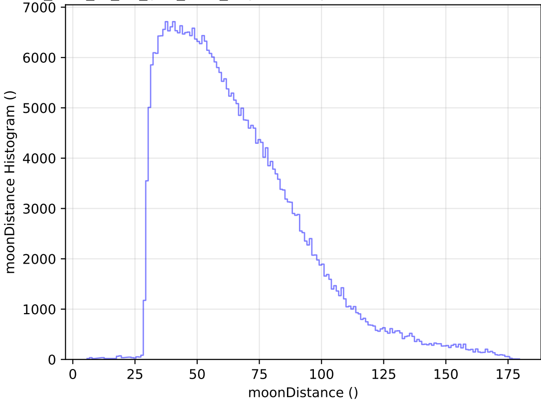
too_elab_r8_d3_griz_v3.4_10yrs WFD y band: moonDistance Histogram
