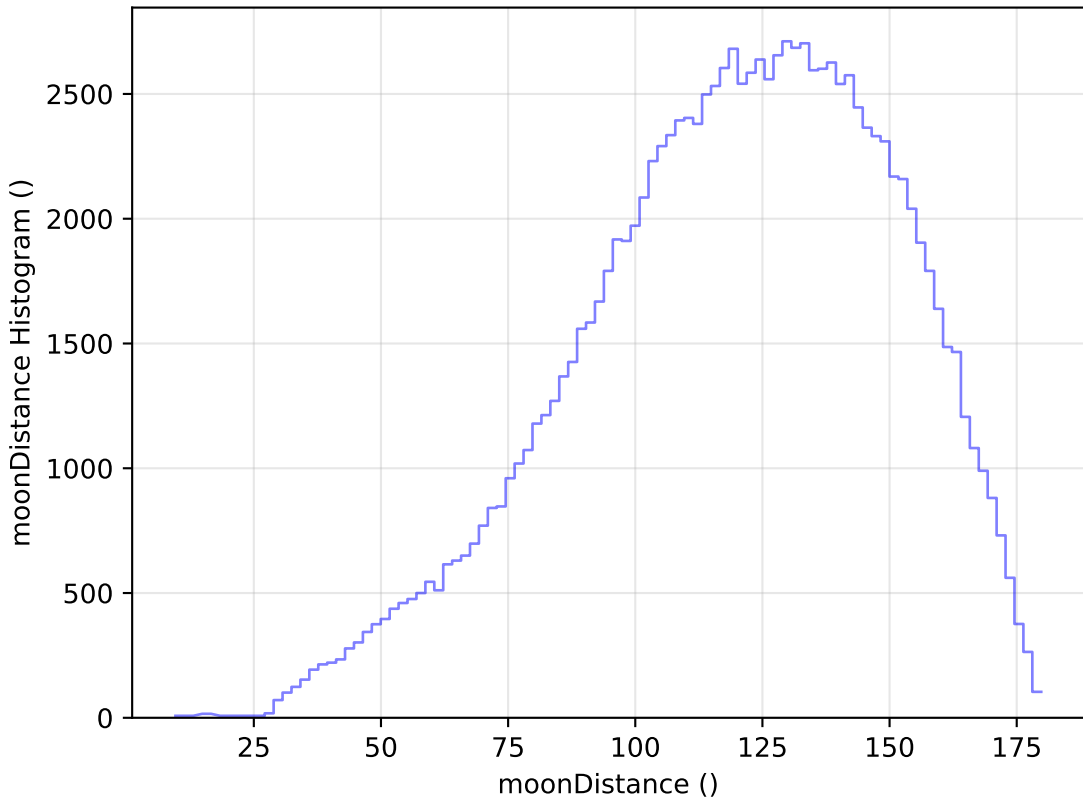
too_elab_r8_d3_griz_v3.4_10yrs WFD u band: moonDistance Histogram
