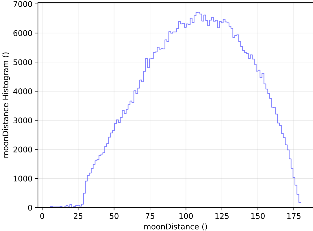
too_elab_r8_d3_griz_v3.4_10yrs WFD r band: moonDistance Histogram
