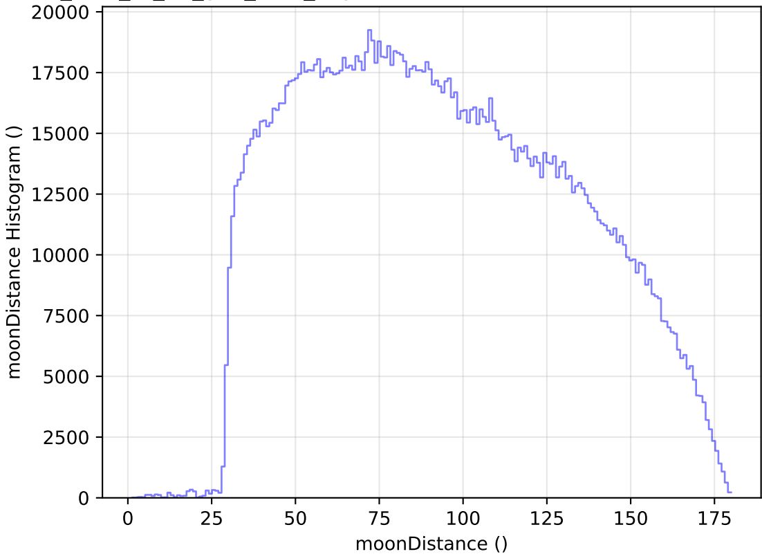
too_elab_r8_d3_griz_v3.4_10yrs WFD all bands: moonDistance Histogram
