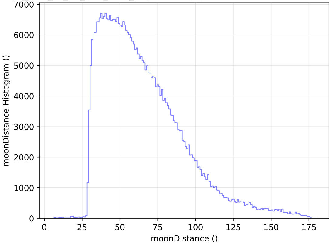
too_elab_r8_d3_griz_v3.4_10yrs All sky y band: moonDistance Histogram
