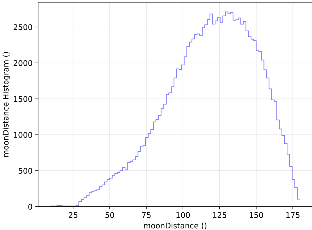
too_elab_r8_d3_griz_v3.4_10yrs All sky u band: moonDistance Histogram
