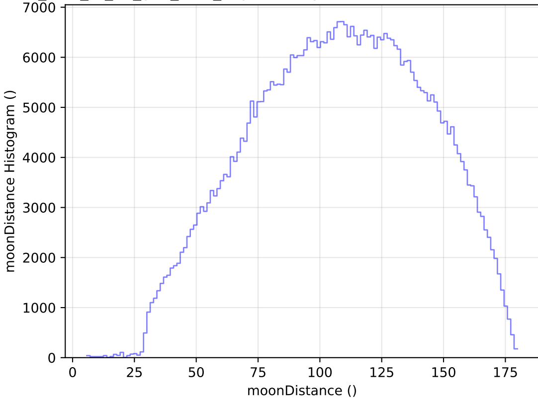
too_elab_r8_d3_griz_v3.4_10yrs All sky r band: moonDistance Histogram
