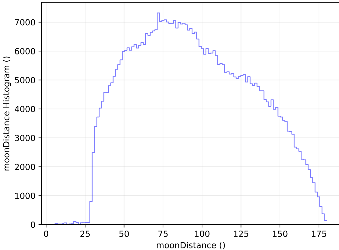
too_elab_r8_d3_griz_v3.4_10yrs All sky i band: moonDistance Histogram
