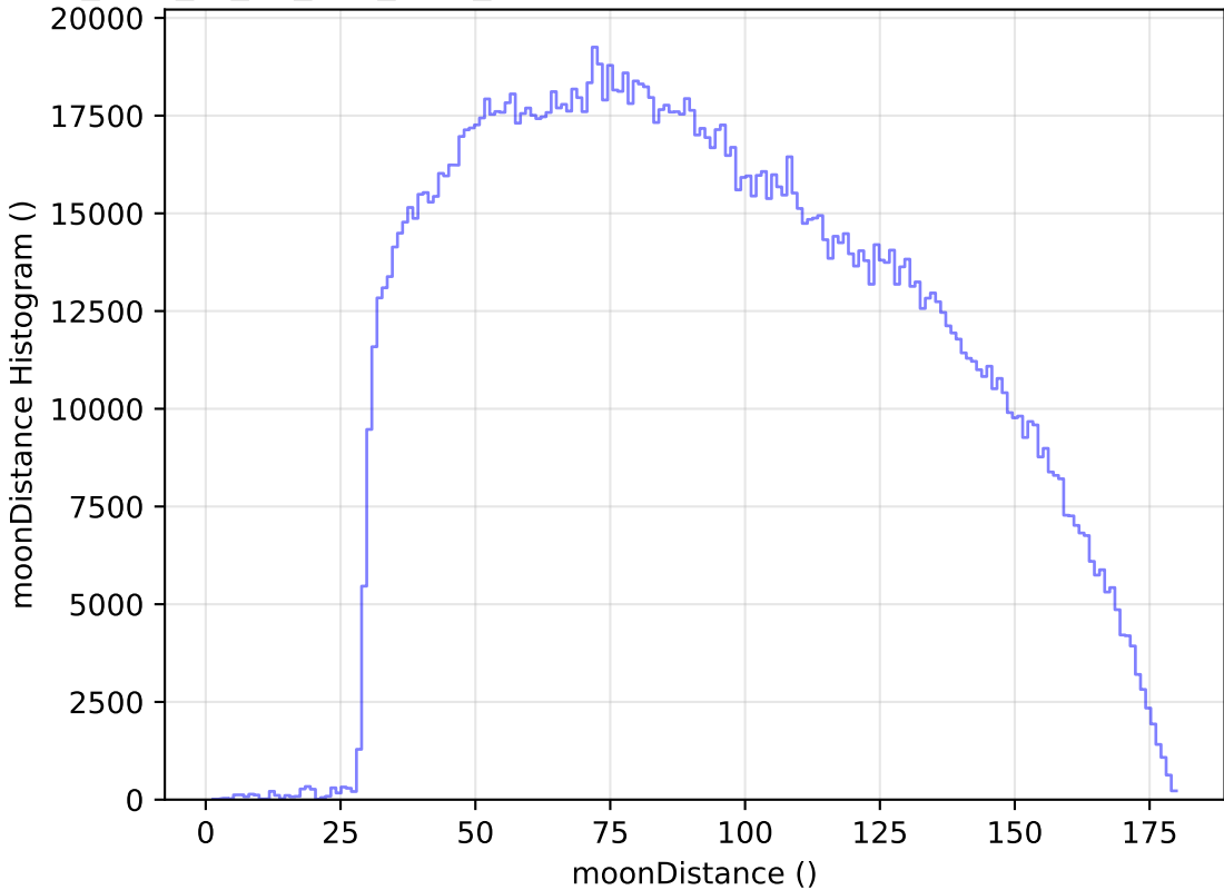
too_elab_r8_d3_griz_v3.4_10yrs All sky all bands: moonDistance Histogram
